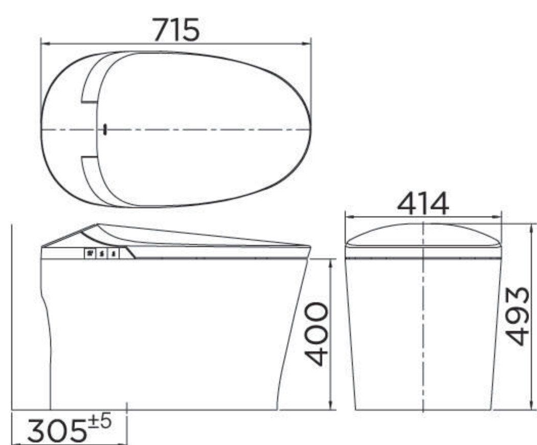
Dimension for ECT-04-120-11(P) , ECT-04-120-55(P) Unit : mm
